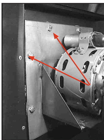
(fig.4) fan mounting plate
