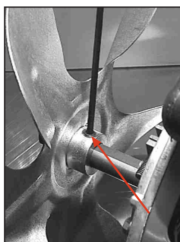
(fig.5) fan blade set screw
