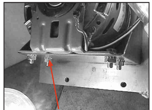
(fig.6) fan motor mounting bolts
