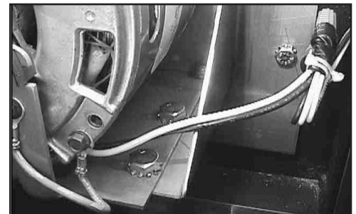
(fig.2) wirenuts connecting fan motor
